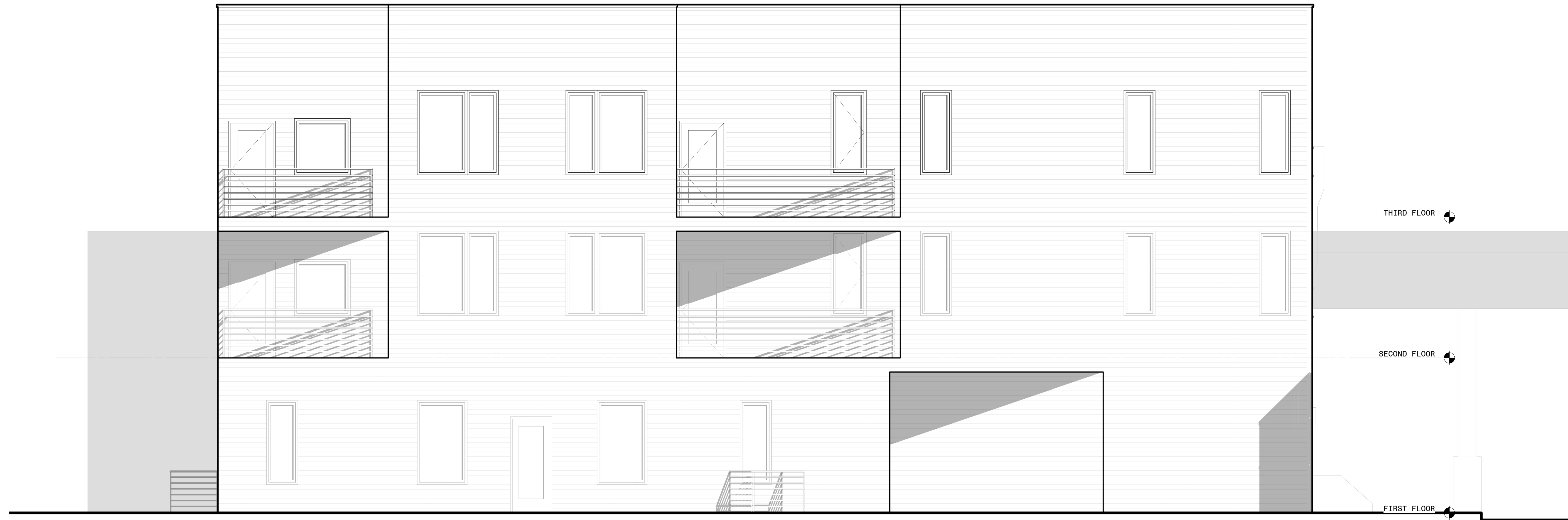
1 EAST ELEVATION 1/4" = 1'-0"
