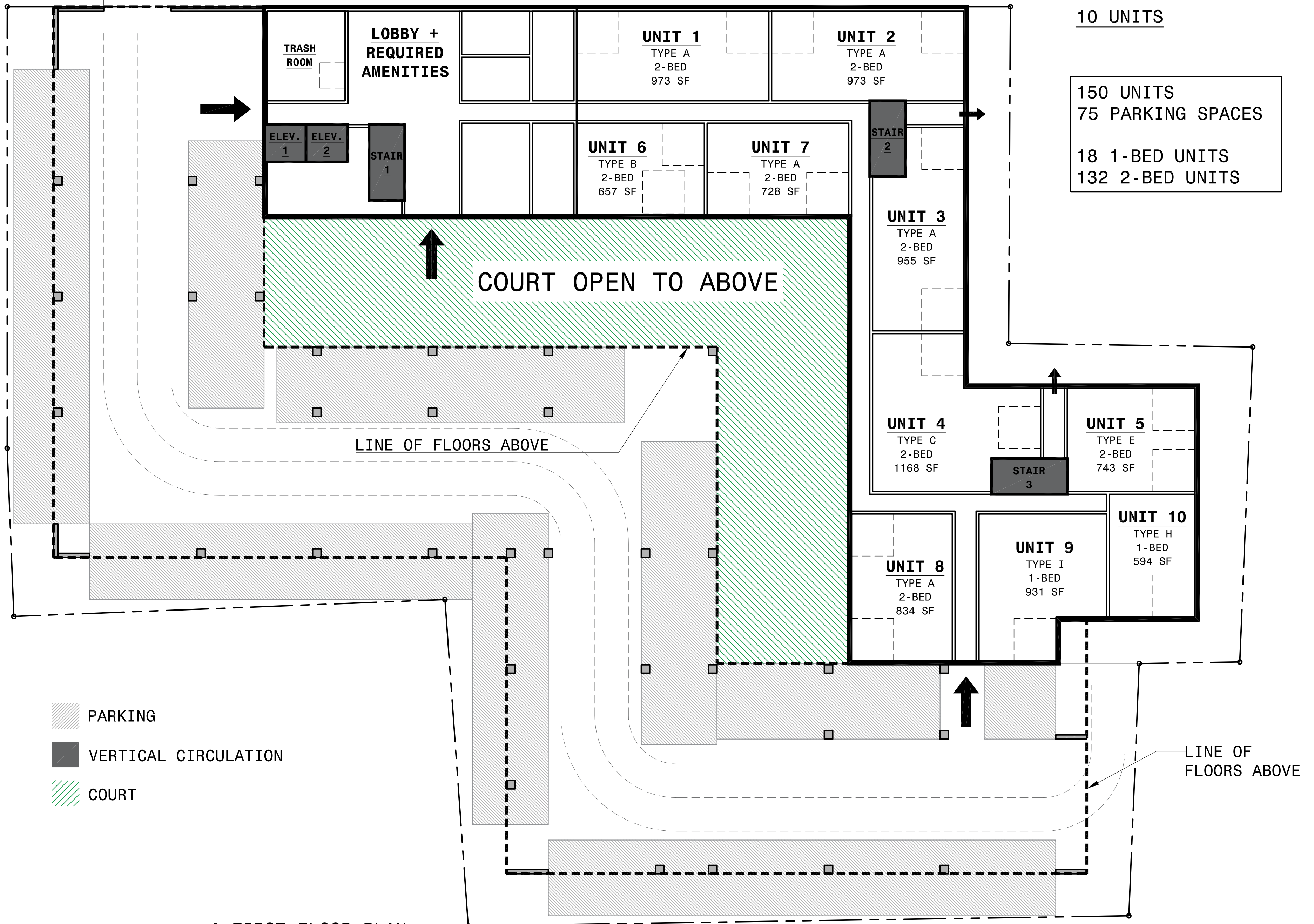
1 FIRST FLOOR PLAN 1/16" = 1'-0"
